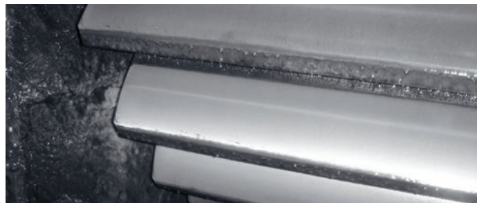
Tooth flanks after repair lubrication
