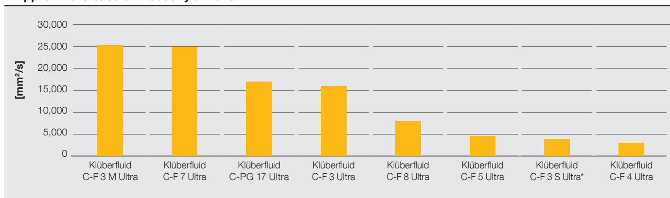
Approximate base oil viscosity at 40 °C
